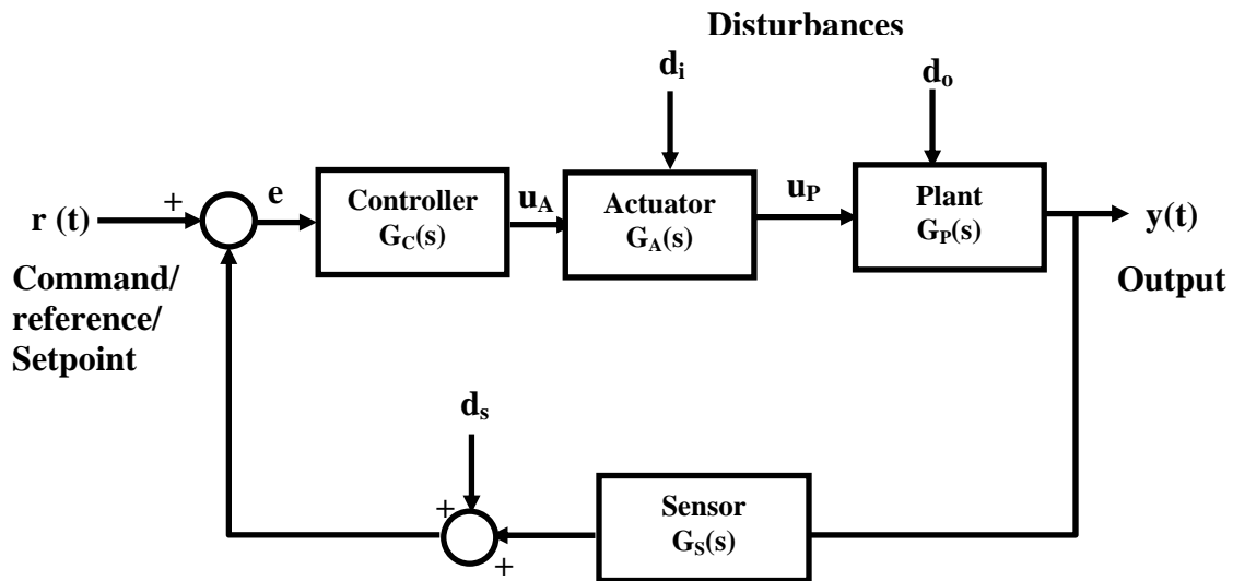
Fig. 2.3 Typical control loop
