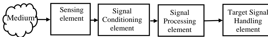
Fig. 2.1 Functional configuration of a typical sensor system
