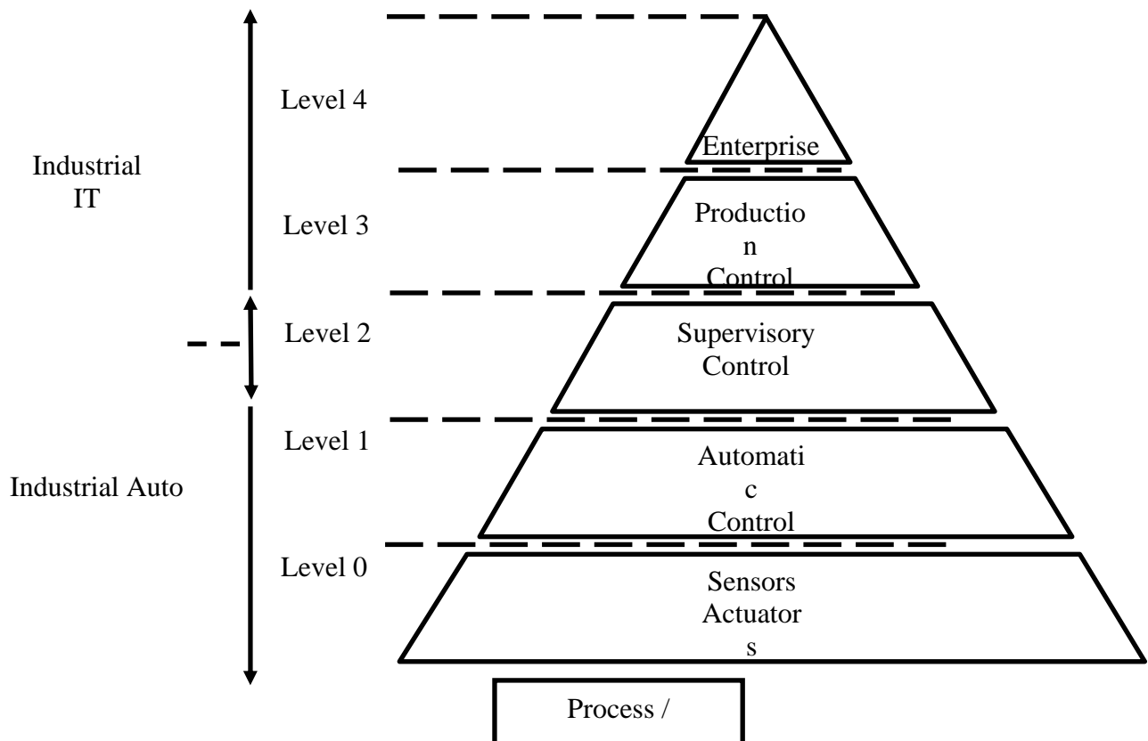
Fig. 2.4 Automation pyramid
